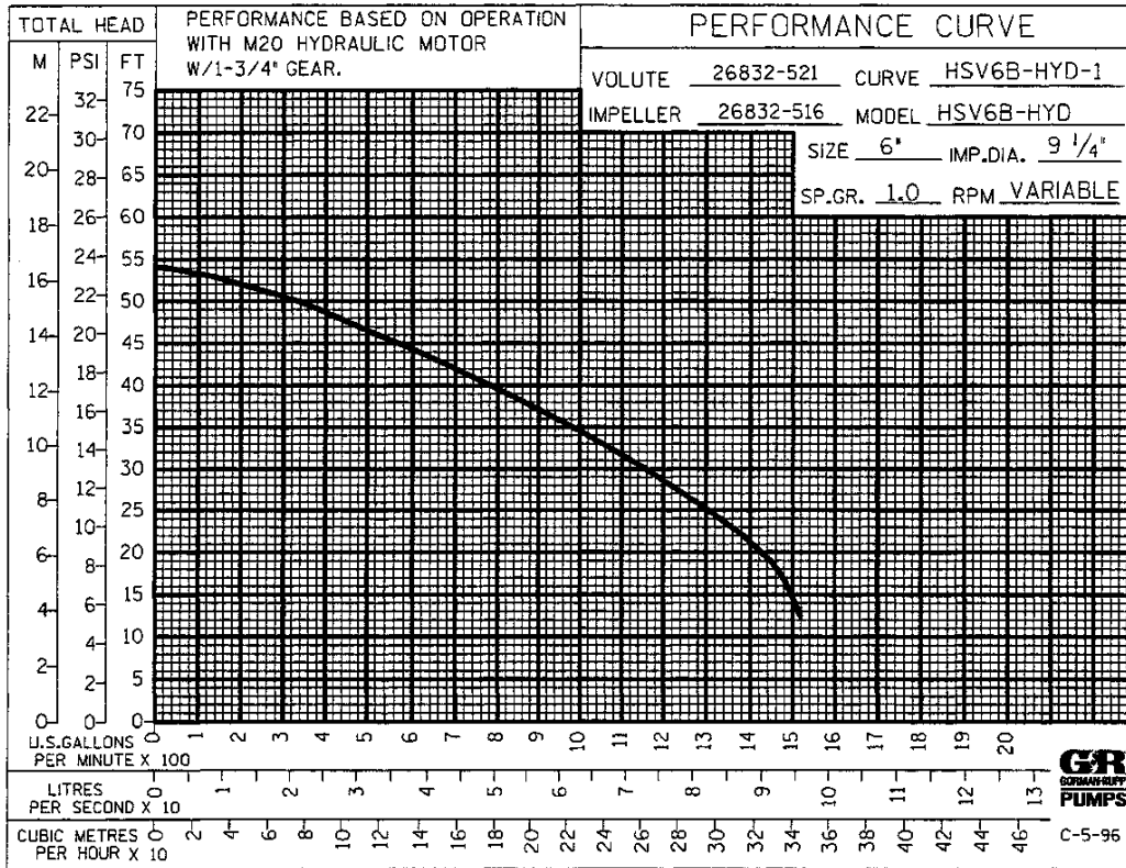
Performance Curve – Model HSV6B31-HYD
