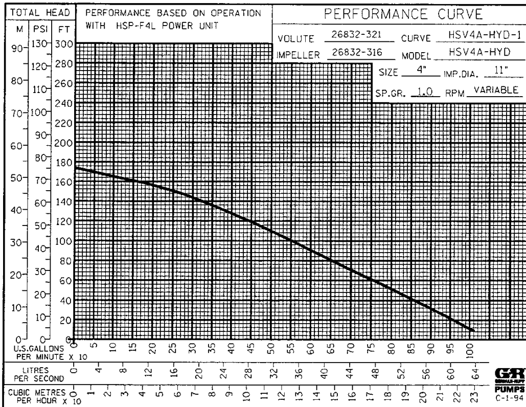
Performance Curve - Model HSV4A31-HYD
